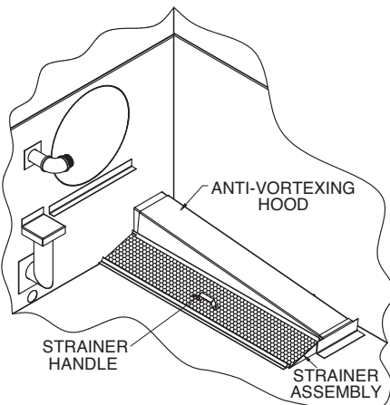
Figure 10 – LSWB/LSC-E/PMC-E/PMWQ Strainer Assembly
