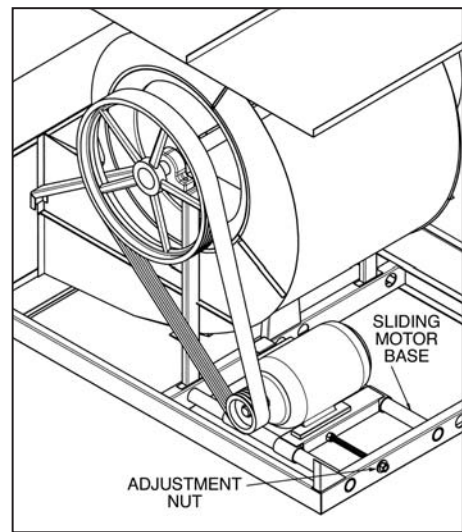
Figure 6 – LR Motor Adjustment
